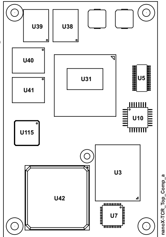
Figure 2-3. Component Locations (Top Side)
