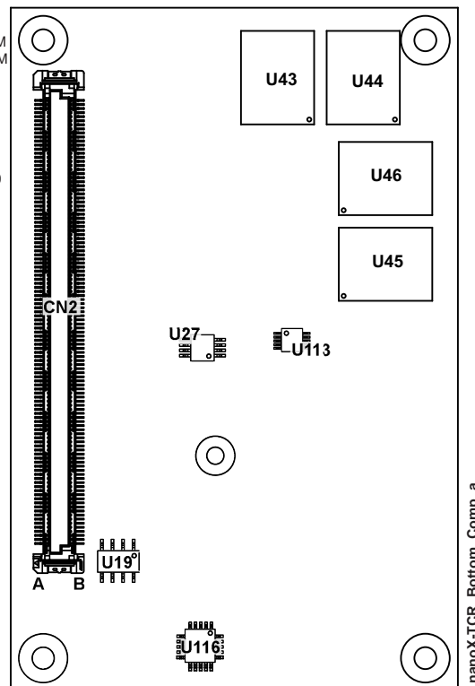
Figure 2-4. Component Locations (Bottom Side)
